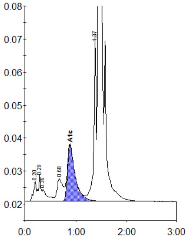
Peak table - ID: 11412843
