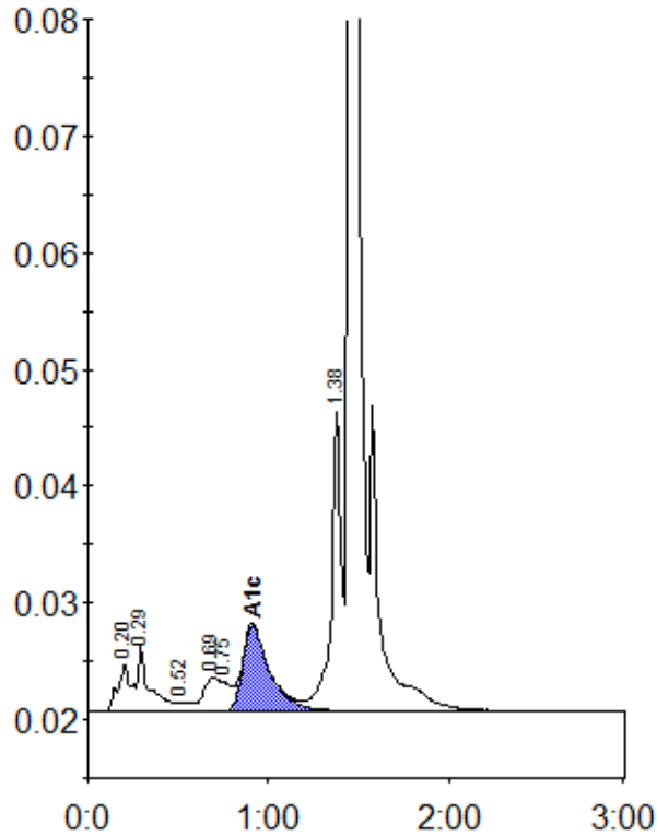
Peak table - ID: 11307422
