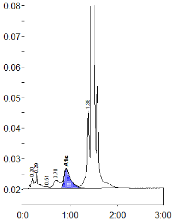
Peak table - ID: 11169939
