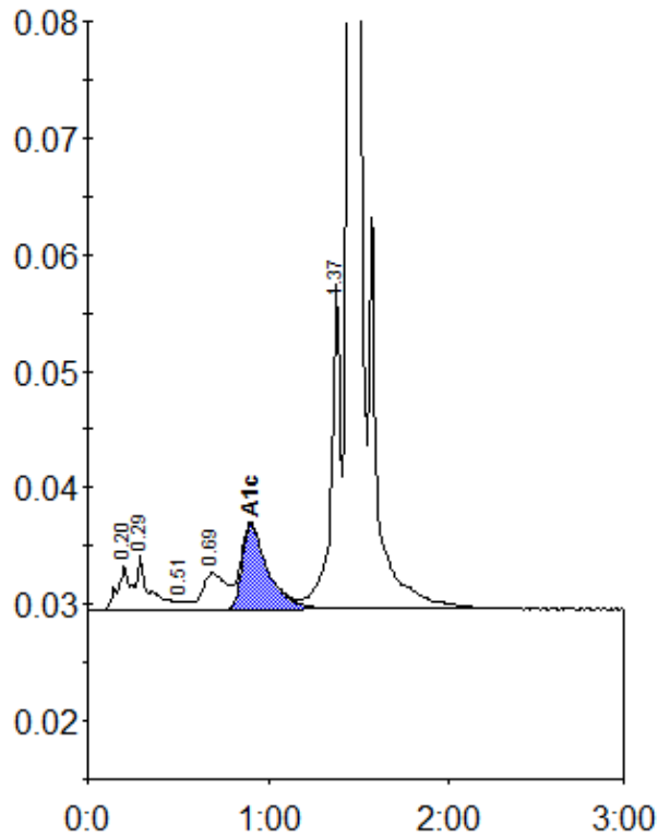
Peak table - ID: 11358822
