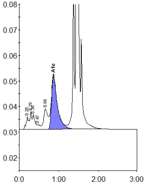
Peak table - ID: 10988730
