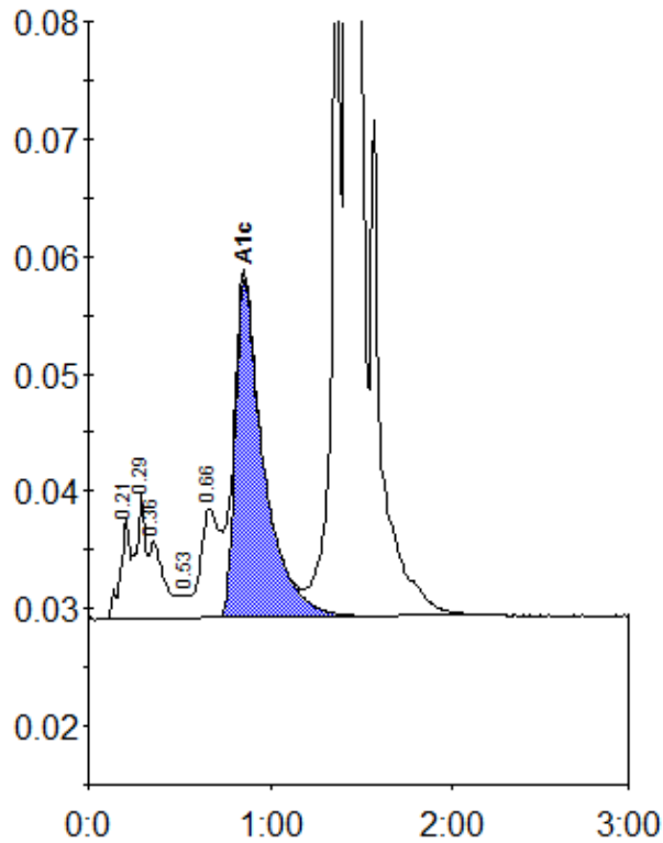
Peak table - ID: 11217958
