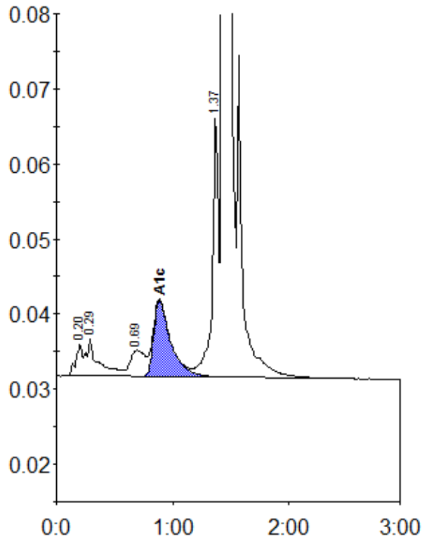
Peak table - ID: 11187937
