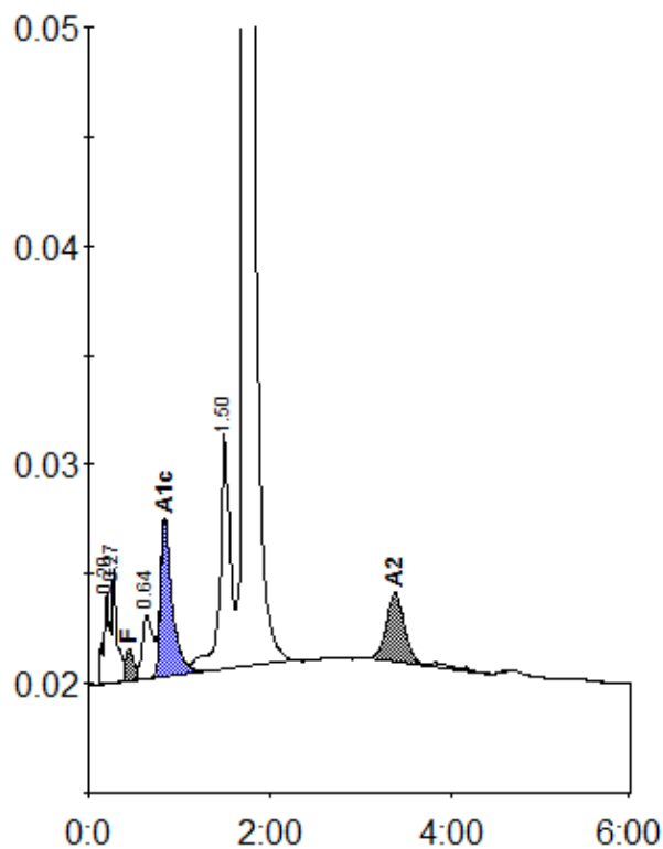
Peak table - ID: 11272850
