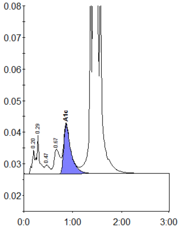
Peak table - ID: 11307633
