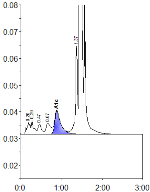
Peak table - ID: 11153514
