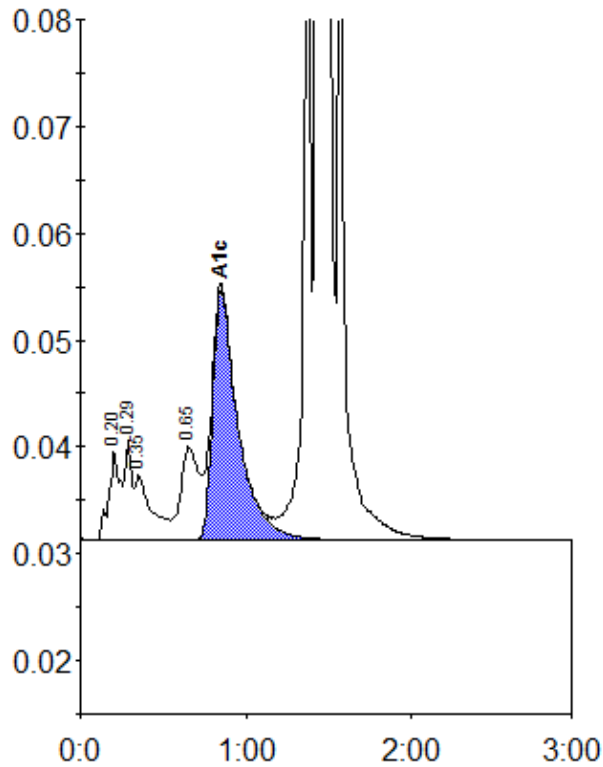
Peak table - ID: 11166901
