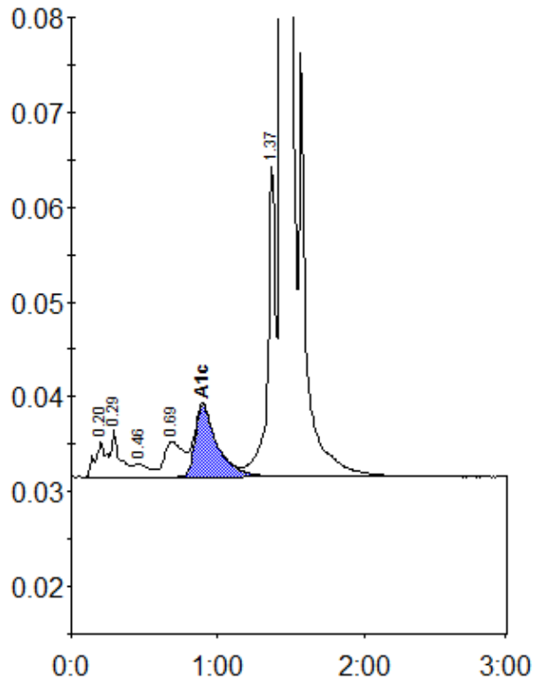
Peak table - ID: 11178376
