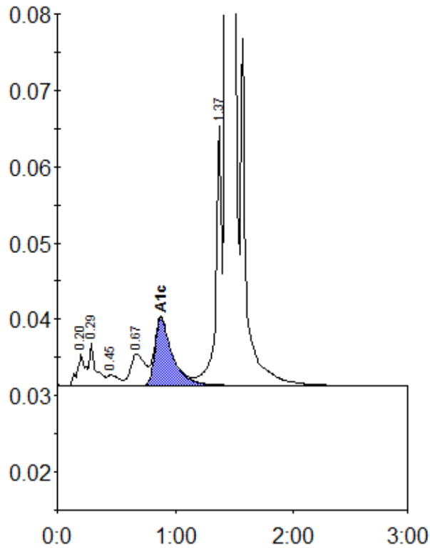
Peak table - ID: 11283277
