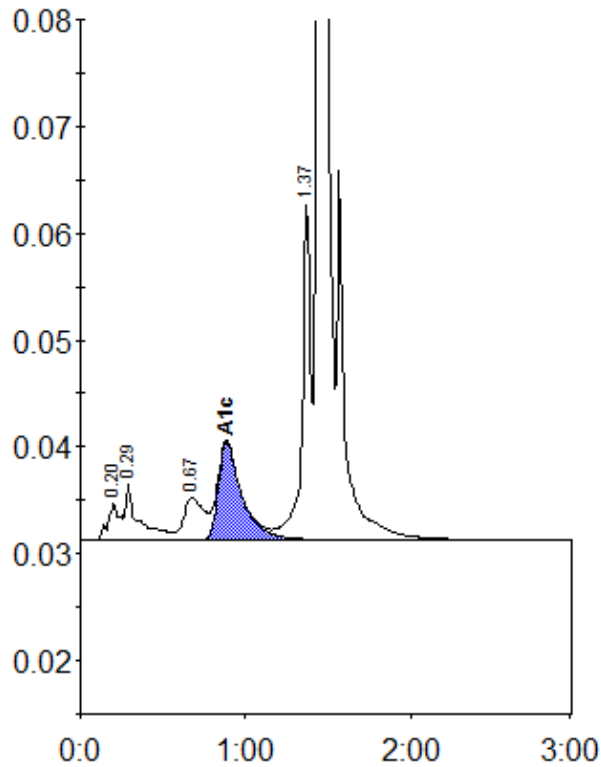
Peak table - ID: 11272420
