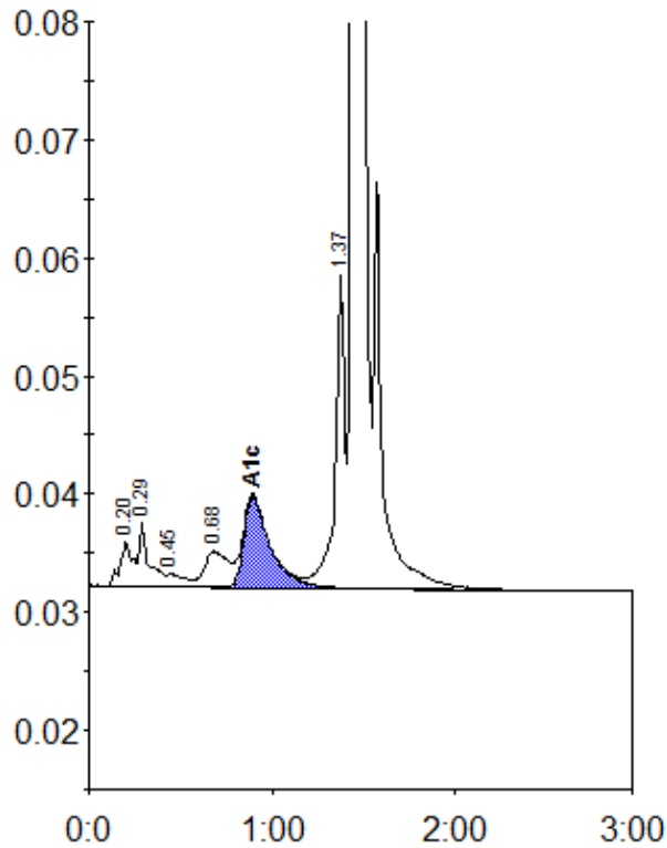
Peak table - ID: 11166837
