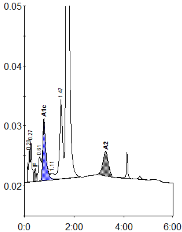
Peak table - ID: 11022372
