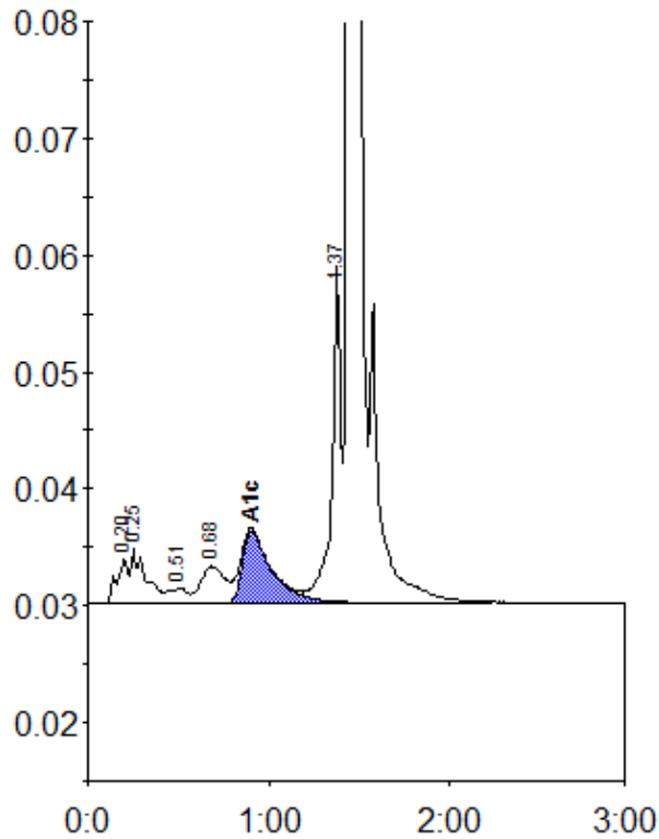
Peak table - ID: 11178054
