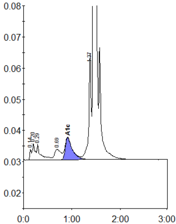
Peak table - ID: 11301514
