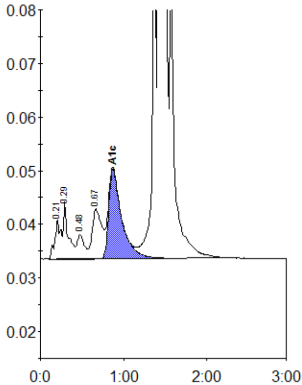
Peak table - ID: 11277908
