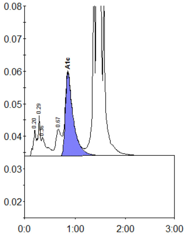
Peak table - ID: 11283740
