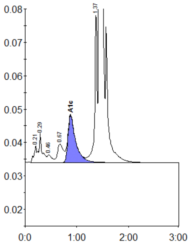
Peak table - ID: 11086380
