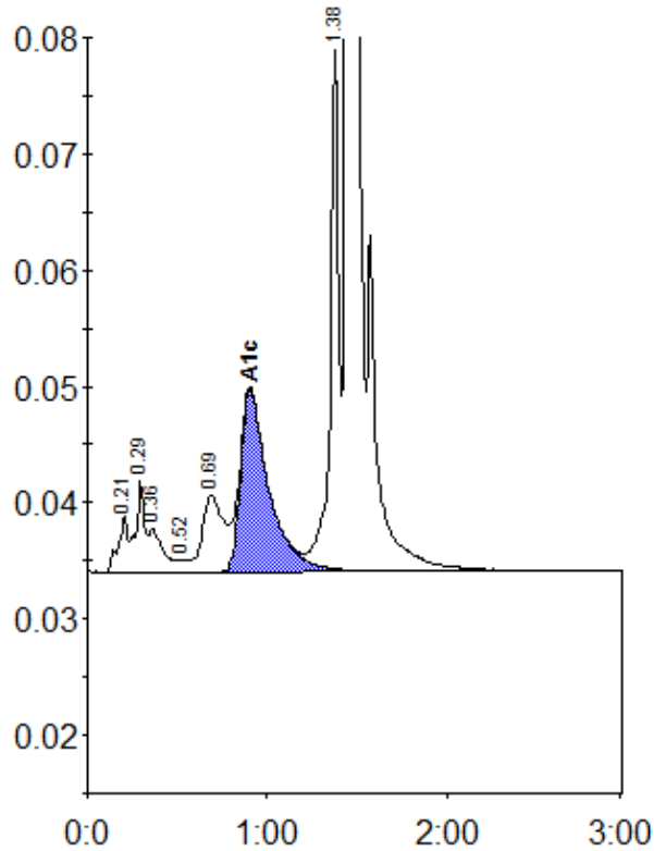
Peak table - ID: 11199868
