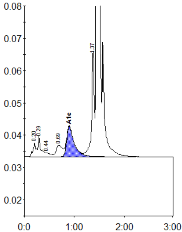
Peak table - ID: 11166880
