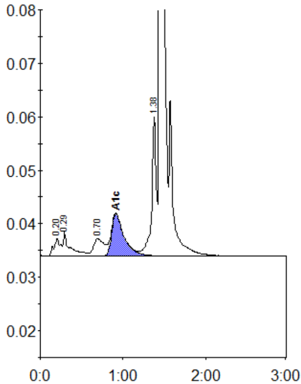
Peak table - ID: 11086432
