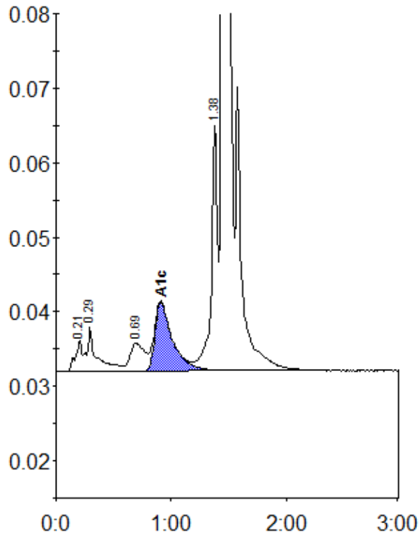
Peak table - ID: 11293044
