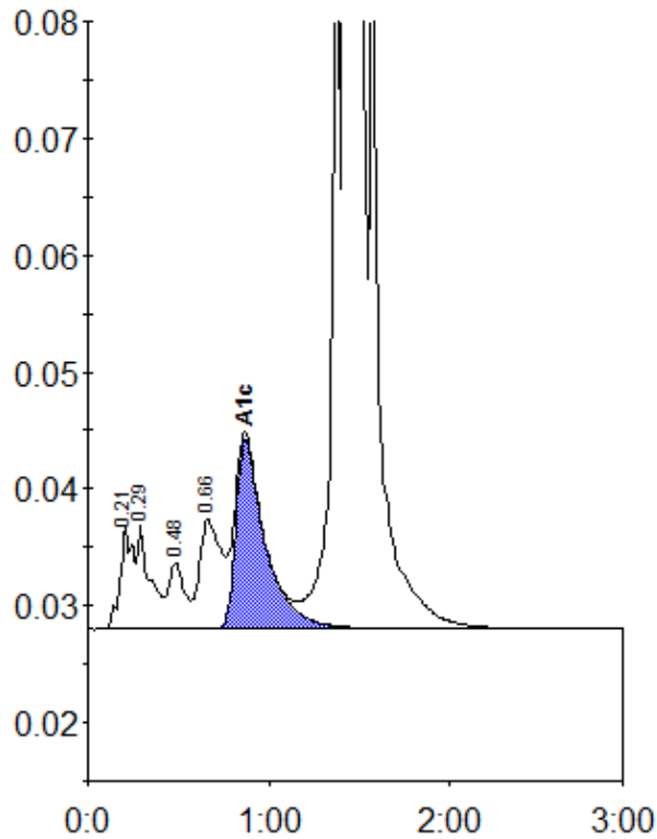
Peak table - ID: 11157146
