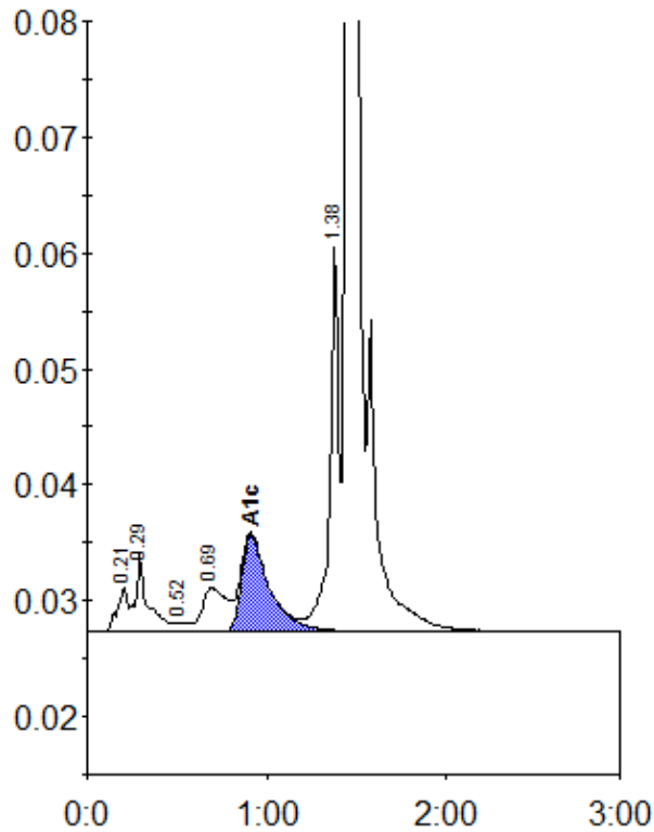
Peak table - ID: 11283504
