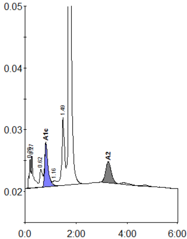
Peak table - ID: 11293280
