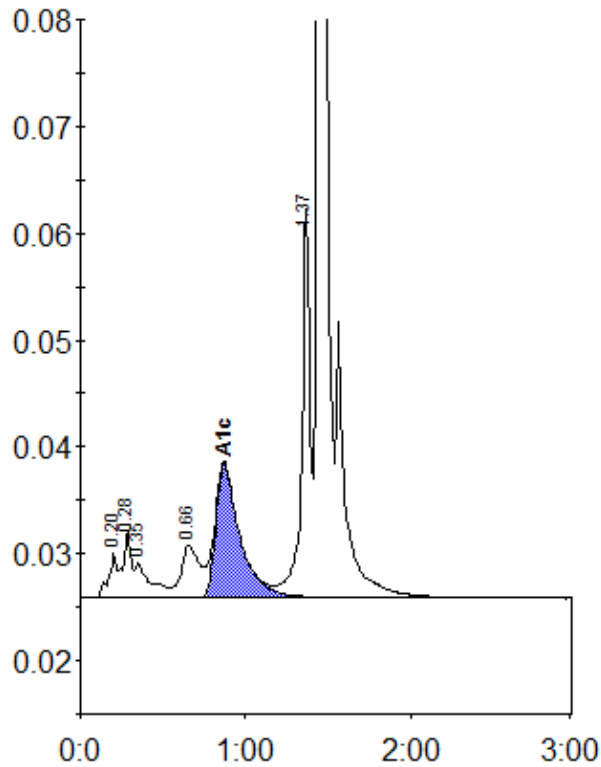
Peak table - ID: 11325012
