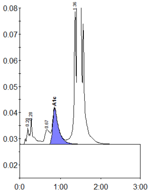
Peak table - ID: 11140428
