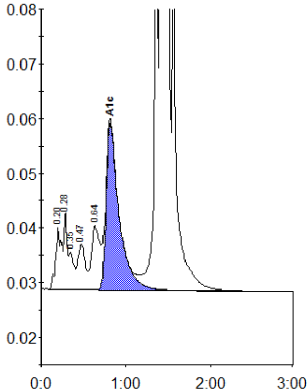
Peak table - ID: 11140553
