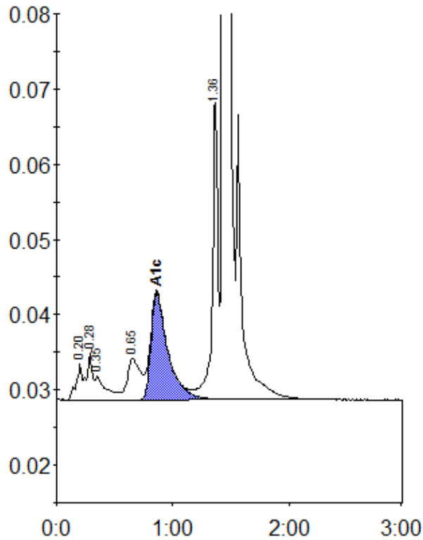
Peak table - ID: 11320567
