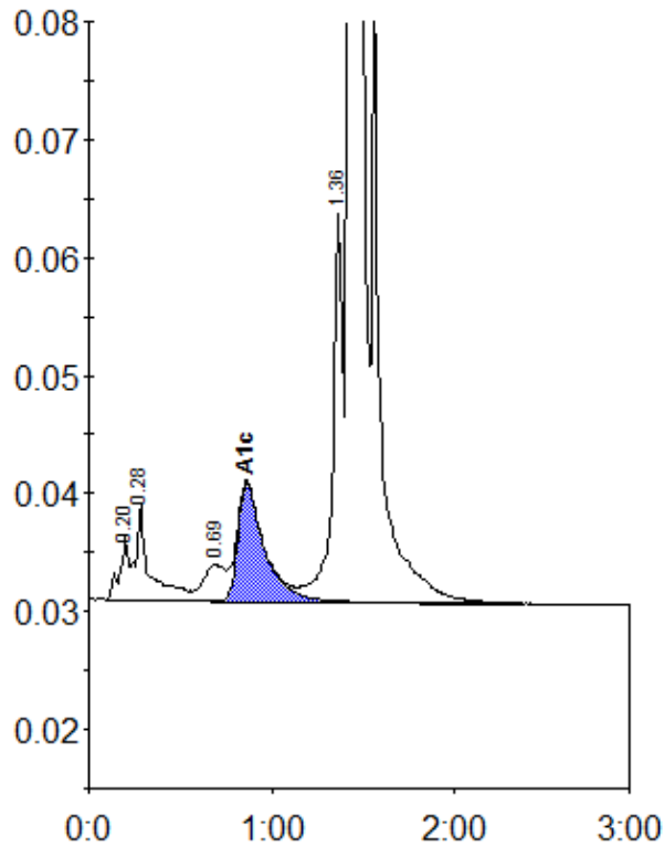
Peak table - ID: 11063395
