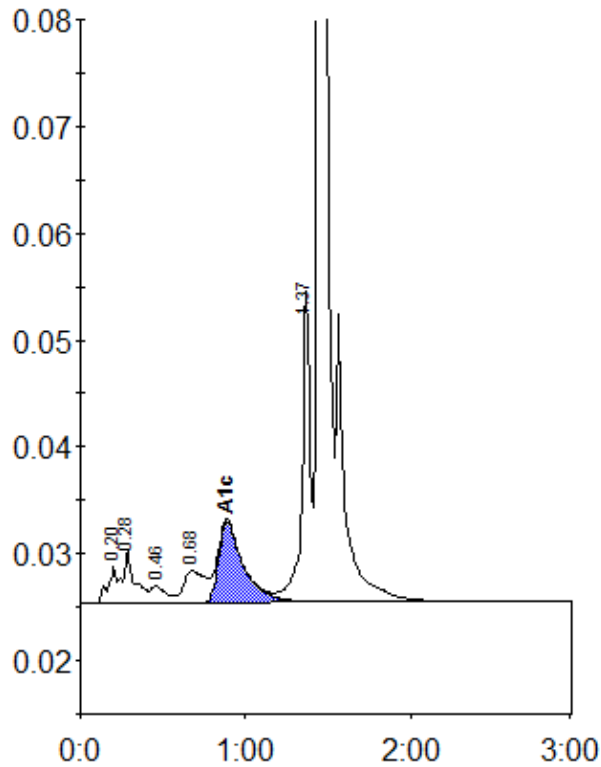
Peak table - ID: 11322258
