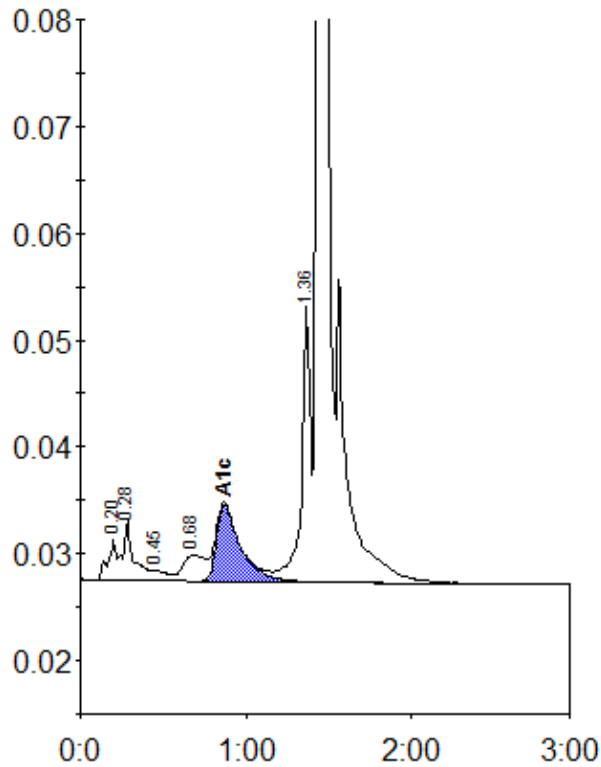
Peak table - ID: 11063419
