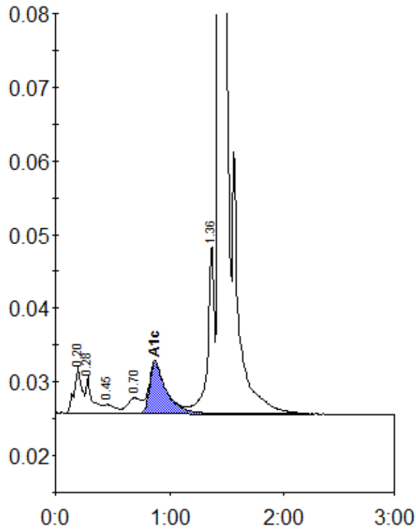
Peak table - ID: 11063424
