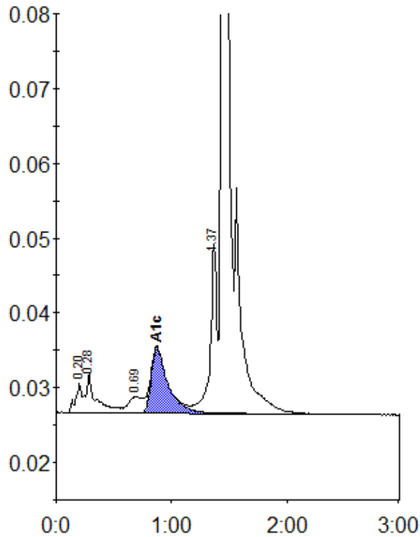
Peak table - ID: 11063428
