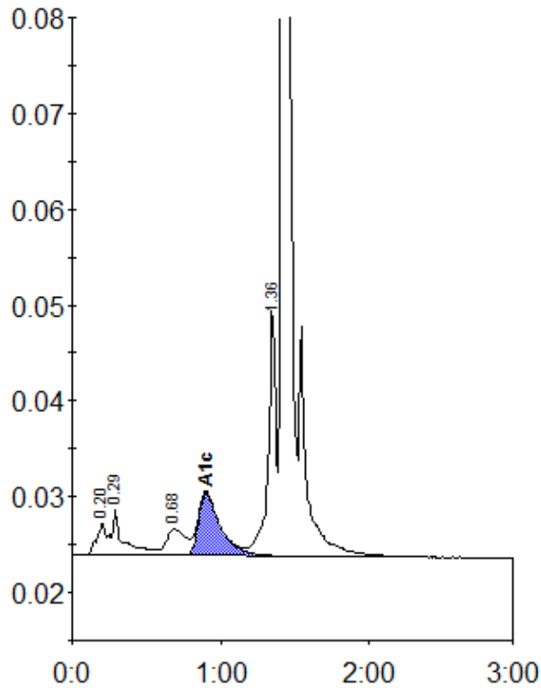
Peak table - ID: 11193849
