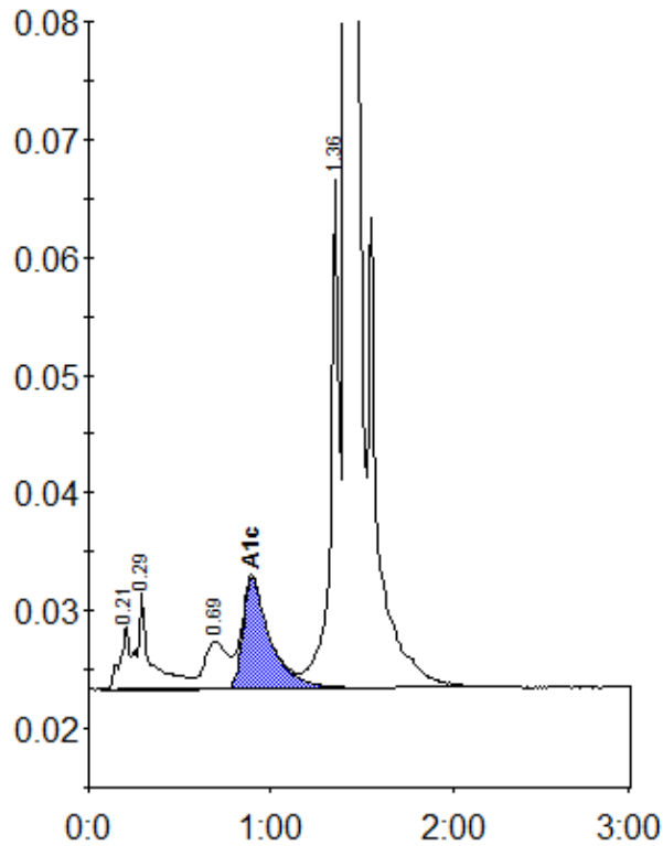
Peak table - ID: 11184617
