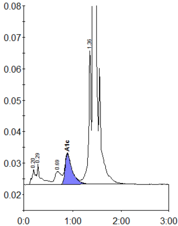
Peak table - ID: 11184620
