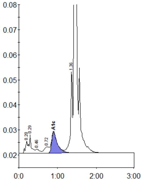
Peak table - ID: 11320622
