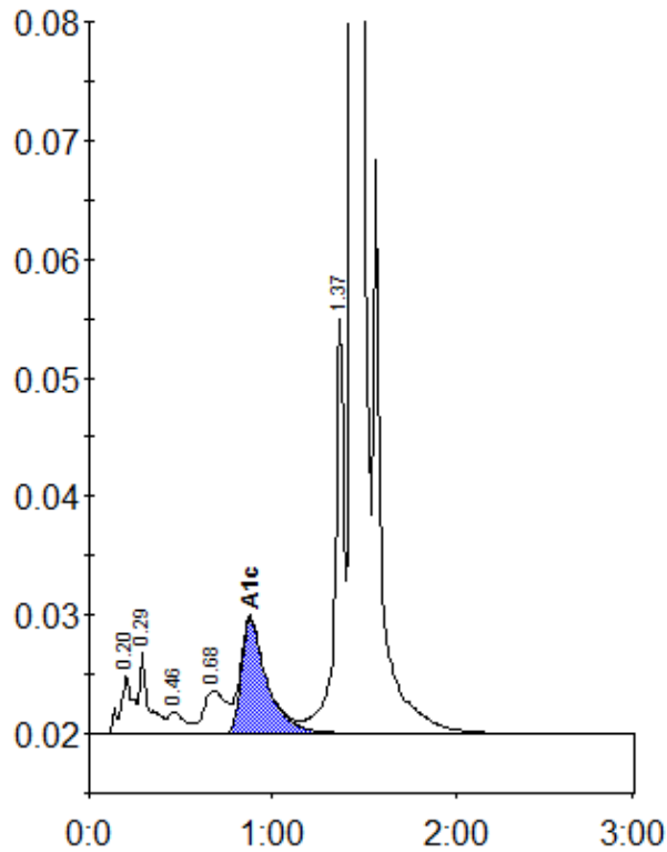
Peak table - ID: 10971910
