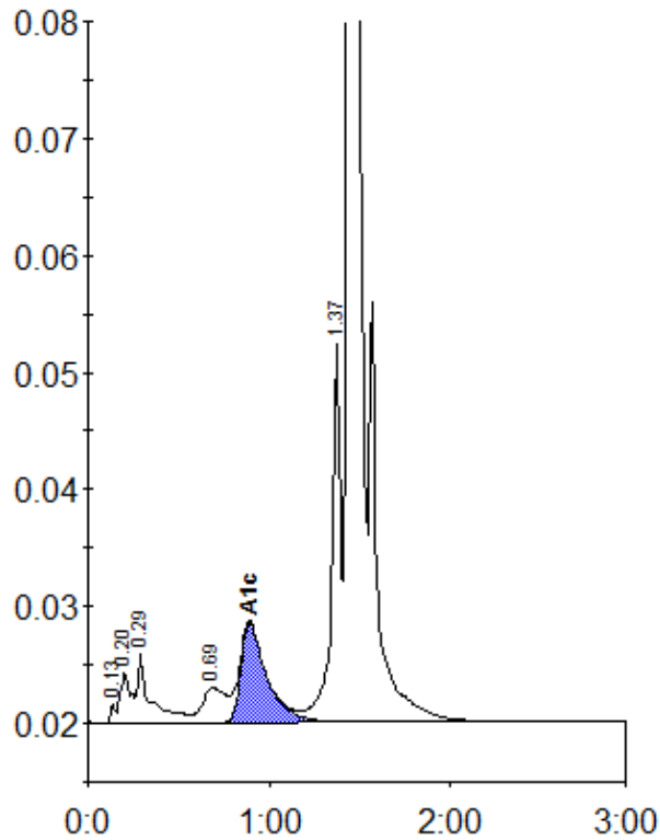
Peak table - ID: 11086714
