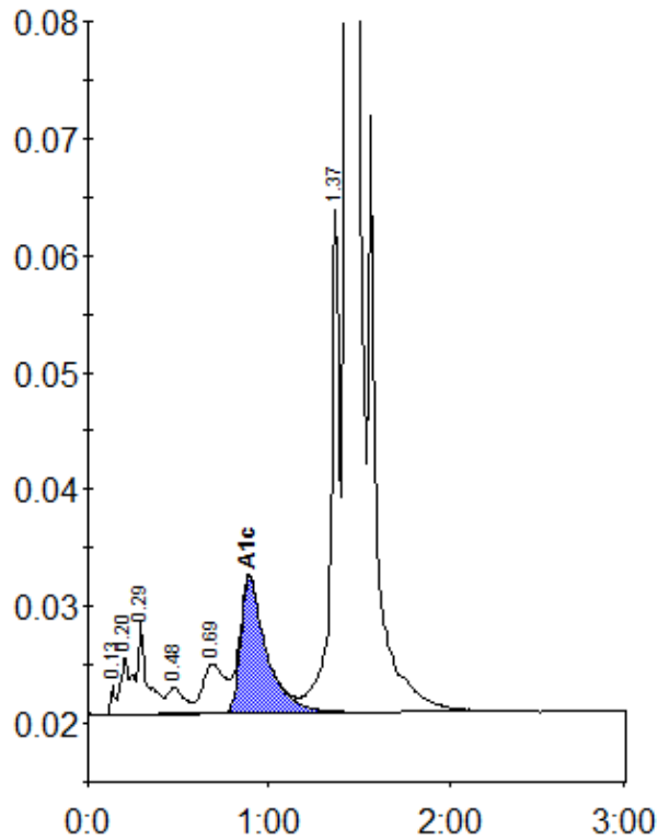
Peak table - ID: 11156215
