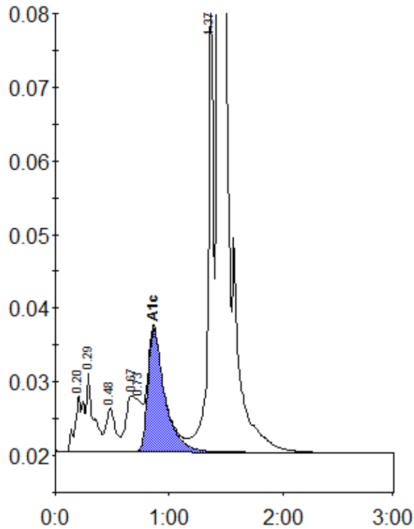
Peak table - ID: 11047629
