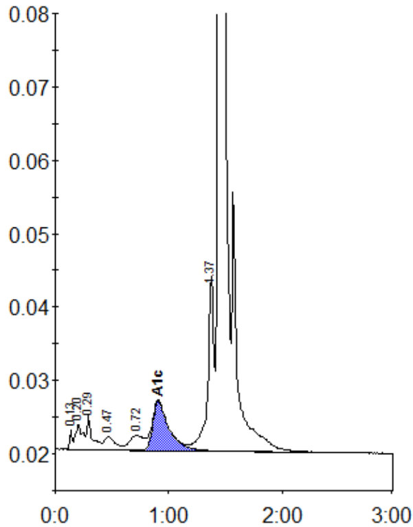
Peak table - ID: 11063645
