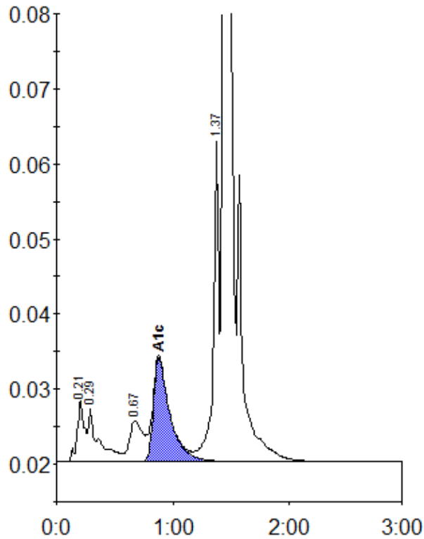
Peak table - ID: 11329952
