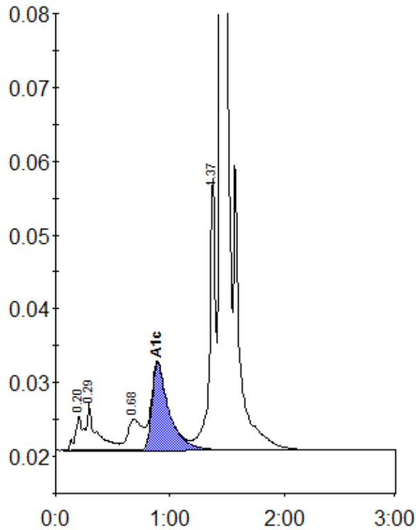
Peak table - ID: 11030695
