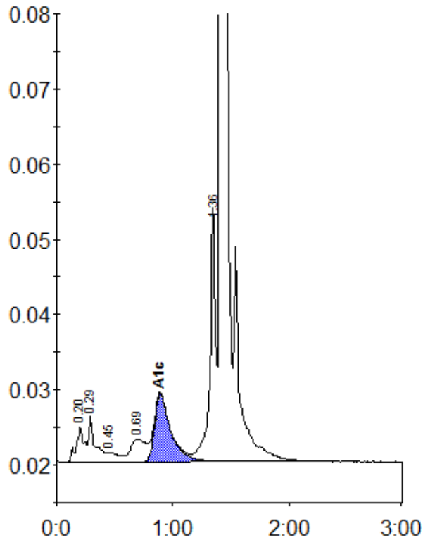
Peak table - ID: 11050990
