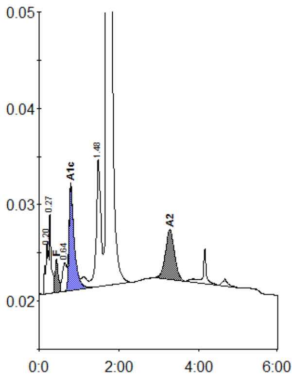
Peak table - ID: 11065485
